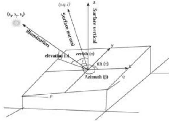
Fig. 1. Specification of solar illumination direction and surface gradients.
